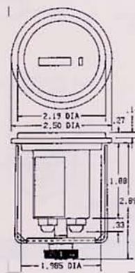
Flush Mount (Stirrup) 2.5": Panel cutout 2.00 diameter opening. *
