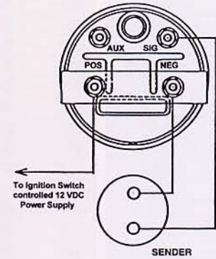
ELECTRIC SPEEDOMETER MAGNETIC PICK UP
