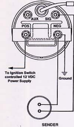
ELECTRIC TACHOMETER MAGNETIC PICK UP
