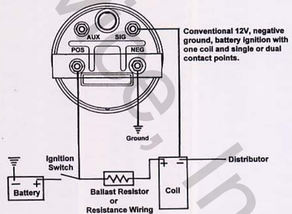
ELECTRIC TACHOMETER GASOLINE
