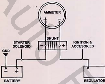
AMMETER (SHUNTED)
