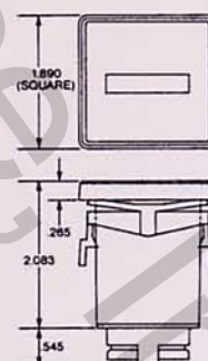
Square Retainer: Panel cutout 1.45 x .95 rectangular opening
