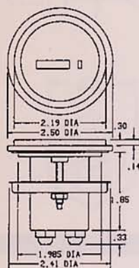
Flush Mount (Cup) 2.5": Panel cutout 2.00 diameter opening. *
