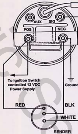
ELECTRIC TACHOMETER HALL EFFECT SENDER
