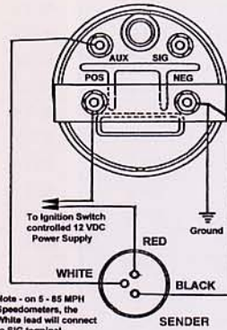
ELECTRIC SPEEDOMETER HALL EFFECT
